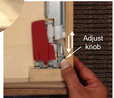
▶ Figure 4. Adjust slides
