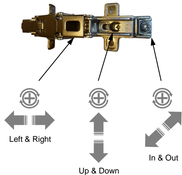
▶ Figure 5. Adjust the door(s) by turning the screws on the hinge.
