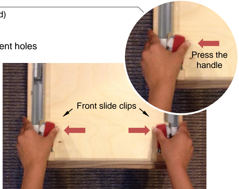
Figure 1. Release the slides
